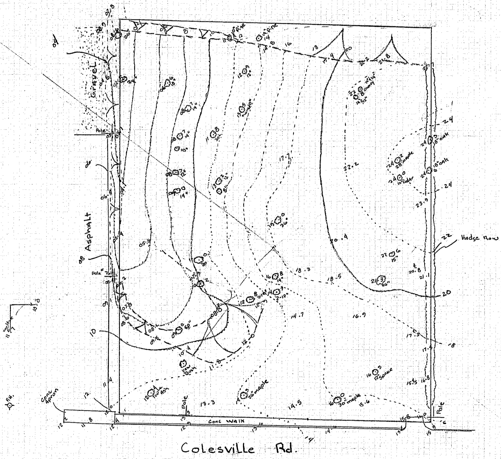
ELLsworth Dr. Urban Park Scale 1" = 30' Feb. 86
