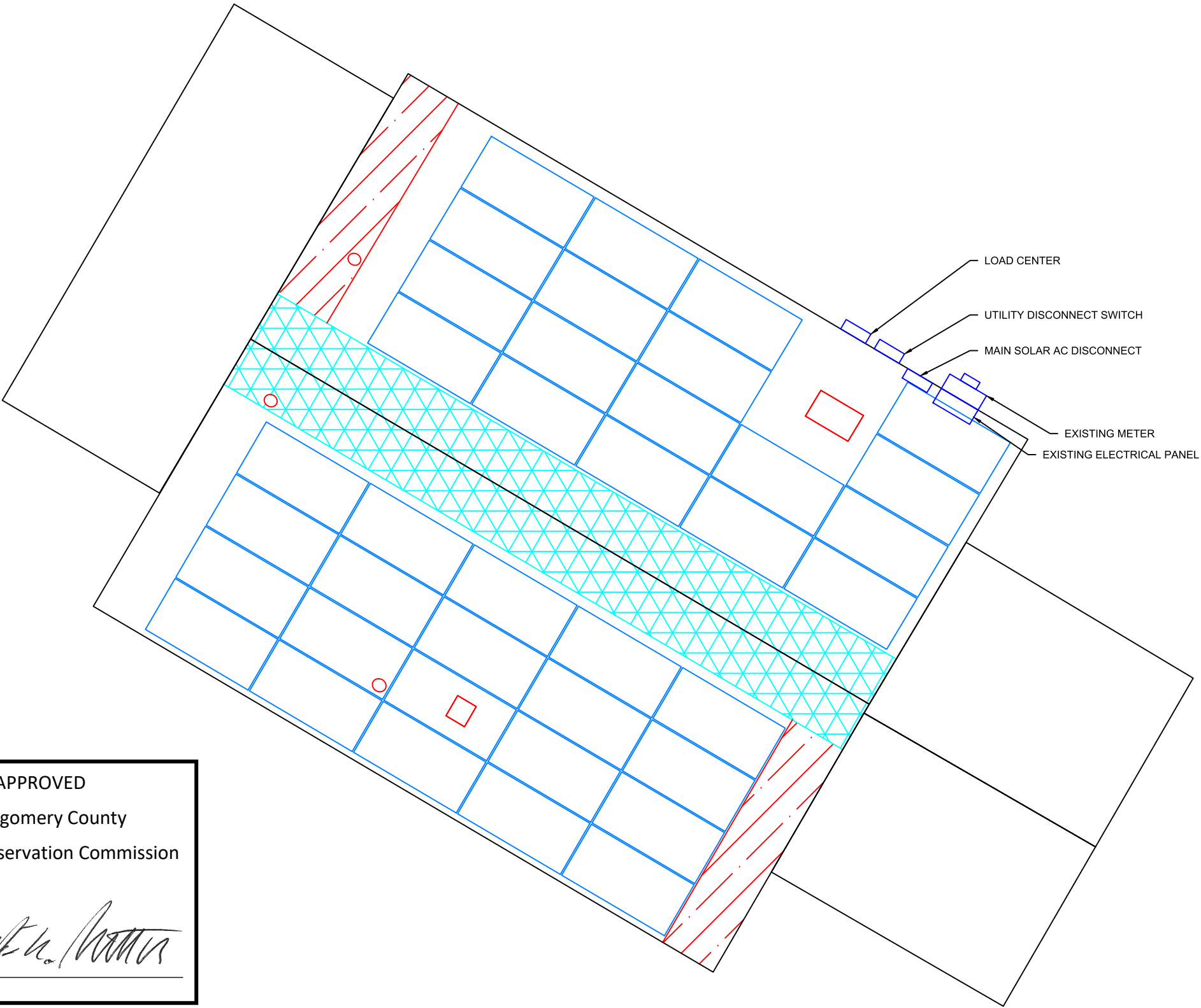
EQUIPMENT LOCATION PLAN Scale: NTS
