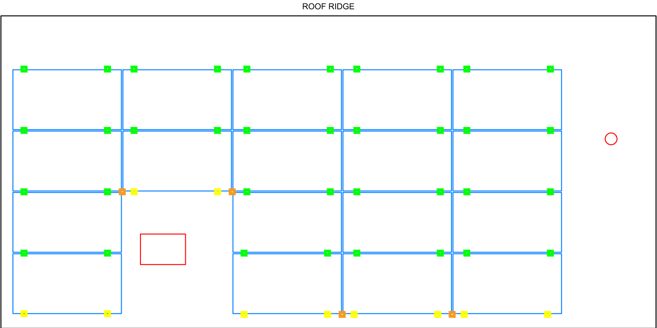
SOLAR PANEL FOOTING PLAN R2 Scale: 3/16" = 1'-0"
