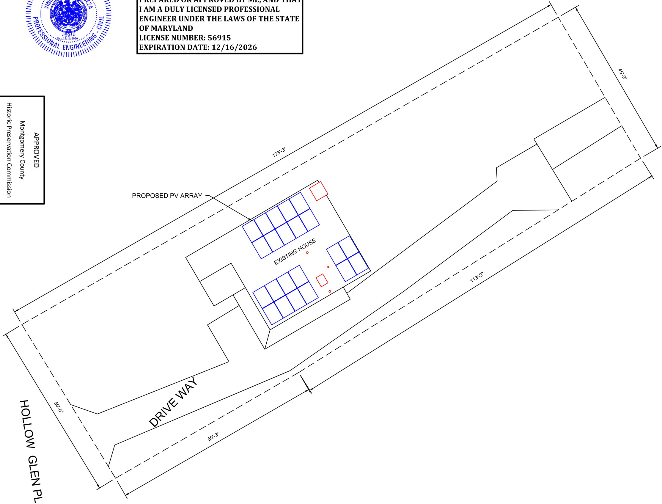
SITE PLAN Scale: 1/16" = 1'-0"
