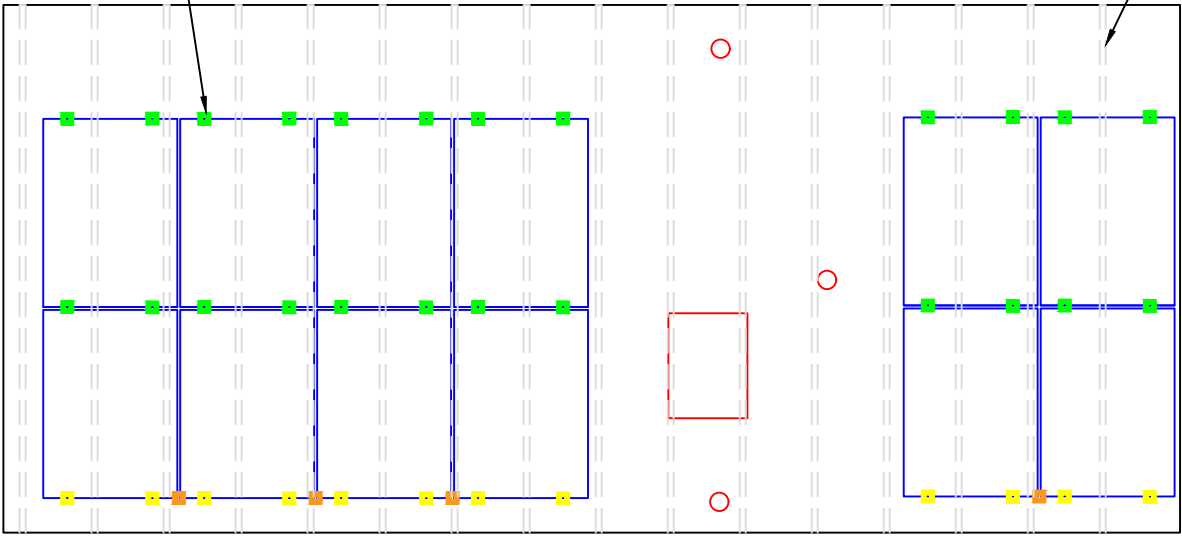
SOLAR PANEL FOOTING PLAN R1
